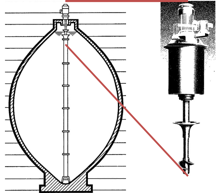
TYPICAL MIXER INSTALLATION
