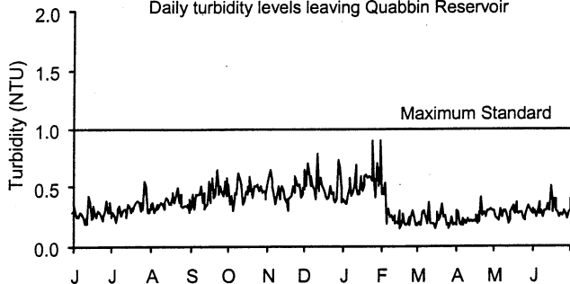
Winsor Power Station, Quabbin Reservoir Daily turbidity levels leaving Quabbin Reservoir
