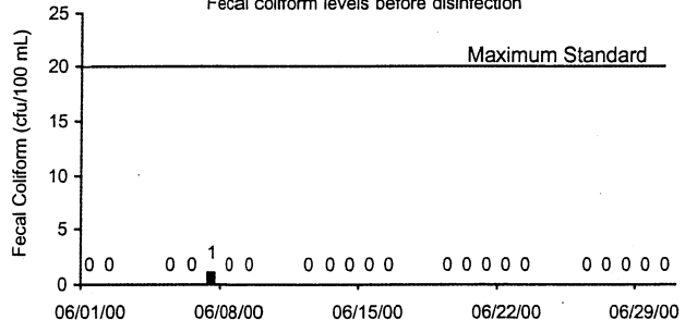
Winsor Power Station, Quabbin Reservoir Fecal coliform levels before disinfection
