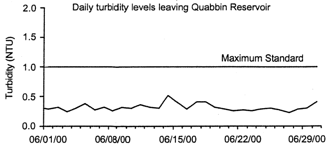
Winsor Power Station, Quabbin Reservoir Daily turbidity levels leaving Quabbin Reservoir
