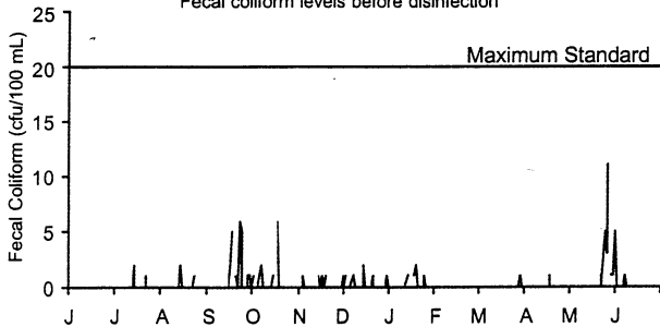
Winsor Power Station, Quabbin Reservoir Fecal coliform levels before disinfection
