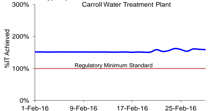
Cryptosporidium IT Percent Achieved - Current Month Carroll Water Treatment Plant
