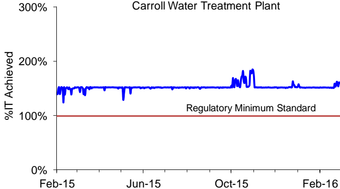
Cryptosporidium IT Percent Achieved - 12 Months Carroll Water Treatment Plant
