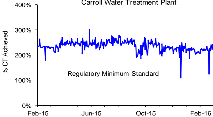
Giardia CT Percent Achievement - 12 Months Carroll Water Treatment Plant
