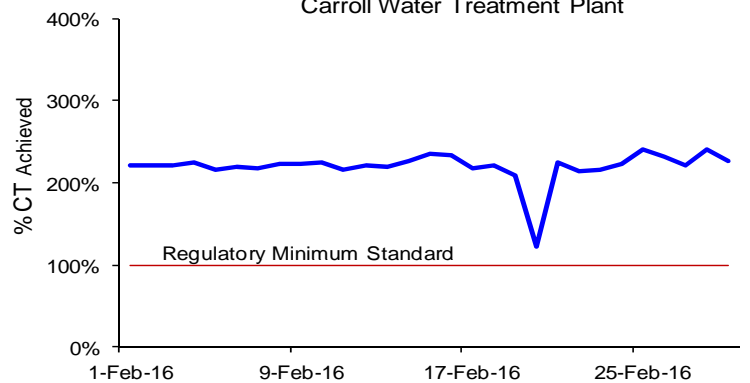
Giardia CT Percent Achievement - Current Month Carroll Water Treatment Plant
